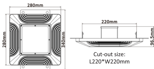
WSLI-CP050/-CP080 (embedded)
