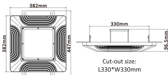
WSLI-CP100/-CP150 (embedded)
