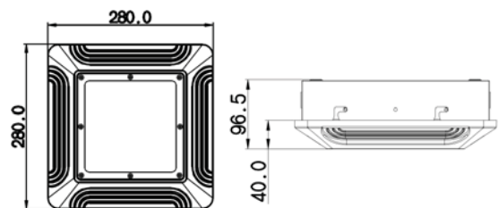
WSLI-CP050/-CP080 (ceiling)
